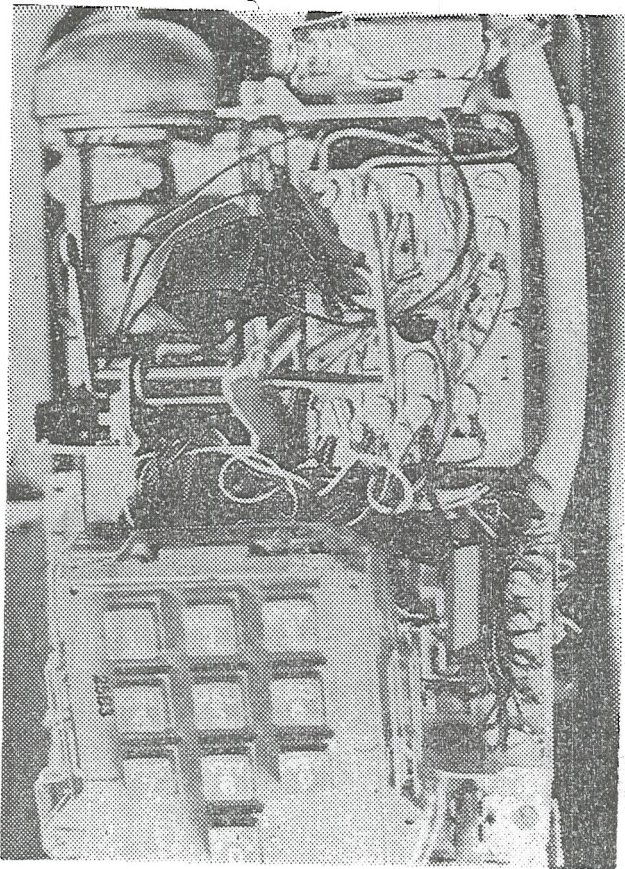
BUG REPORTED: Photograph of the inside of the telephone of Spencer Oliver, executive director of the State Chairmen's Association of the Democratic National Committee. The black rectangular object near the top center of the instrument was found when security men from the Chesapeake and Potomac Telephone Company opened the telephone at request of Mr. Oliver's office.
