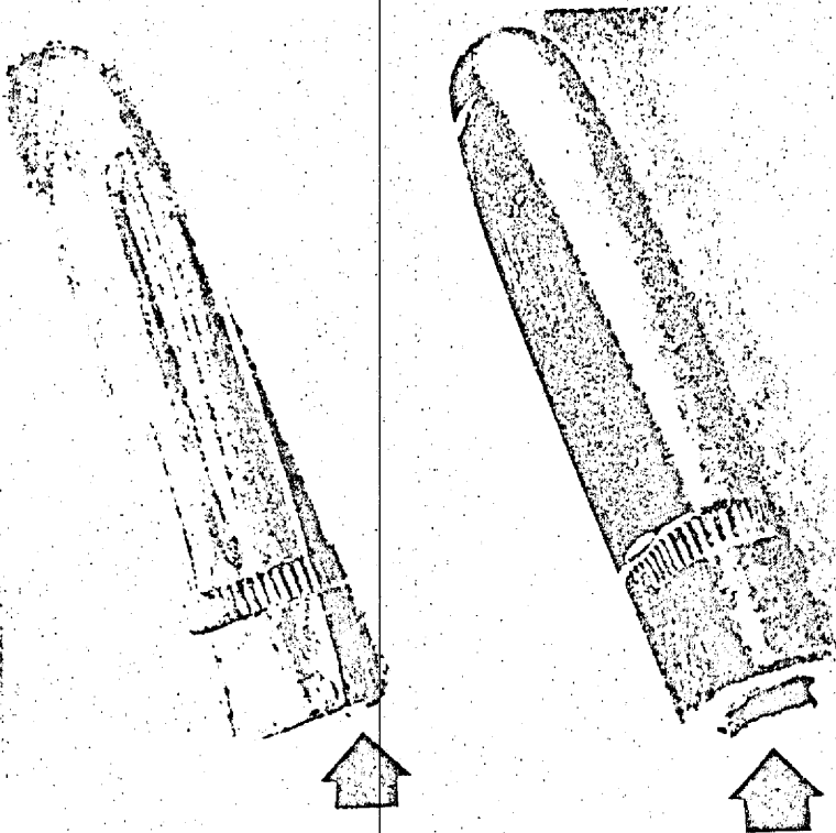
Fig. 1. —Test bullet (right) has been flattened the same amount as bullet 399 (left), even though the flattening of bullet 399 does not show in this view. Note the portion of lead "core" extruded (arrow, right) from rear end of test bullet, caused by this flattening. Only a tiny amount of extruded "core" remains, protruding from the base of bullet 399 (arrow, left). The rest had been scraped off, presumably by its passage through Governor Connally's wrist.
